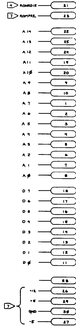
ROM PACK CONNECTOR 30 PIN CONNECTOR
