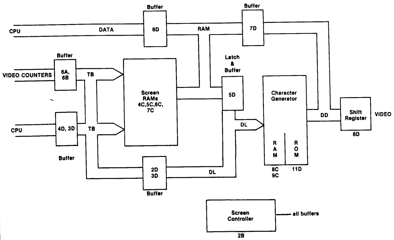
Figure 15. Video Generator Block Diagram
